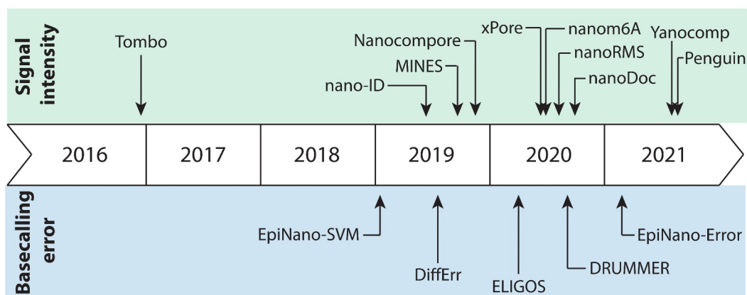
Figure 2. Chronological overview of the community efforts to develop tools to detect and quantify RNA modifications using direct RNA nanopore sequencing.
