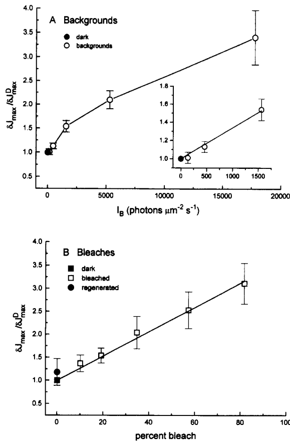
FIGURE 3. Dependence of \delta J_{\text{max}} / \delta J_{\text{max}}^D on background intensity and percent pigment bleached. Values for \delta J_{\text{max}} and \delta J_{\text{max}}^D were obtained for each cell as in Figs. 1 and 2 from the one-third power of the normalized current after stepping into control solution containing 500 \mu\text{M} IBMX. (A) Means \pm SE's of \delta J_{\text{max}} / \delta J_{\text{max}}^D for seven cones in darkness ( \bullet ) and in 600 nm background light ( \circ ). (Insert) \delta J_{\text{max}} / \delta J_{\text{max}}^D in darkness and for the three dimmest backgrounds replotted on expanded axes. Straight line is linear regression constrained to pass through the point ( I_B = 0 , \delta J_{\text{max}} / \delta J_{\text{max}}^D = 1 ). See text. (B) Means \pm SE's of \delta J_{\text{max}} / \delta J_{\text{max}}^D for seven cones in darkness ( \blacksquare ), after a series of bleaches of increasing duration ( \square ), and after regeneration of the photopigment with 11- cis retinal ( \bullet ). Straight line is linear regression constrained to pass through the point (percent bleach = 0, \delta J_{\text{max}} / \delta J_{\text{max}}^D = 1 ). See text.
