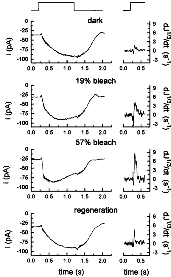
FIGURE 2. Steps into solution containing 500 \mu\text{M} IBMX in darkness, in steady state after exposure to bleaching light, and in steady state after regeneration with exogenous 11- cis retinal. (Left) Current responses to steps from control solution into IBMX under the following conditions (top to bottom): in darkness; 2–3 min after a total of 1 s exposure to a 600-nm light of intensity 3.4 \times 10^7 photons \mu\text{m}^{-2}\text{s}^{-1} , which we estimate to have bleached 19% of the visual pigment; 2–3 min after a total of 4 s exposure to the same 600-nm light, which we estimate to have increased the percentage of pigment bleached to 57%; and 10–11 min after exposure to liposomes containing 11- cis retinal (see Methods). Each response is the average of four measurements. (Right) Derivative of the one-third power of the normalized current for the first 0.6 s of the responses on the left. Uppermost traces give time course of trigger pulses generated by the PCLAMP software (see Fig. 1).
