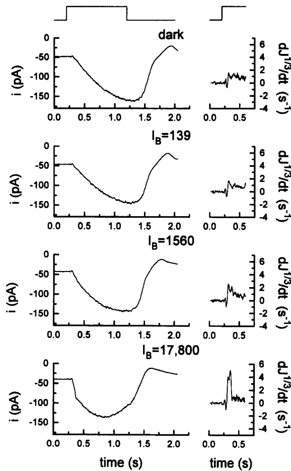
FIGURE 1. Steps into IBMX solution in darkness and in background light. ( Left ) Current responses to steps from control solution into 0.5 mM IBMX solution in darkness and in three backgrounds, as indicated ( I_B = 139 , I_B = 1,560 , and I_B = 17,800 ) in units of photons \mu\text{m}^{-2} \text{s}^{-1} at 600 nm. Each current trace is the average of four measurements. ( Right ) Derivative of the one-third power of the normalized current for the first 0.6 s of the responses on the left. Uppermost traces give time course of triggers generated by PCLAMP software. The \sim 75 ms delay between the onset of the trigger and the beginning of the change in junction current was caused in part by a delay in the microprocessor that generates the signal controlling the stepping motor, coupled to the solution pipette assembly; and in part by the time required for the interface between the control and test solutions to reach the photoreceptor. Current responses have not been corrected for the small junction currents produced by addition of IBMX.
