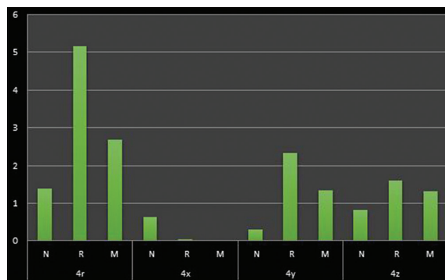
Graph 4: Absolute mean values of deviation for the fourth (4) angulated implant in N, R and M groups from the reference model (x-axis, y-axis, and z-axis in millimeters and “r” in degree)
