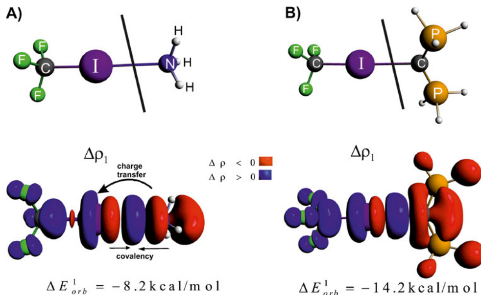
Fig. 2 The contour of deformation density contribution \Delta\rho_1 describing formation of the halogen bonding in 1-NH 3 (part A) and in 1-CPH 3 (part B). In addition the corresponding ETS-NOCV-based energies (in kcal mol -1 ) are shown. The numerically smallest contour values are \pm 0.0005 a.u.
