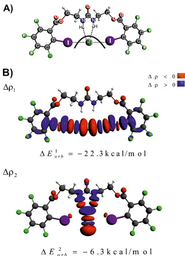
Fig. 5 The contours of deformation density contributions describing the halogen ( \Delta\rho_1 ) and hydrogen bonding ( \Delta\rho_2 ) in 3-Cl . In addition the corresponding ETS-NOCV-based energies (in kcal mol -1 ) are shown. The numerically smallest contour values are \pm 0.0005 a.u.
