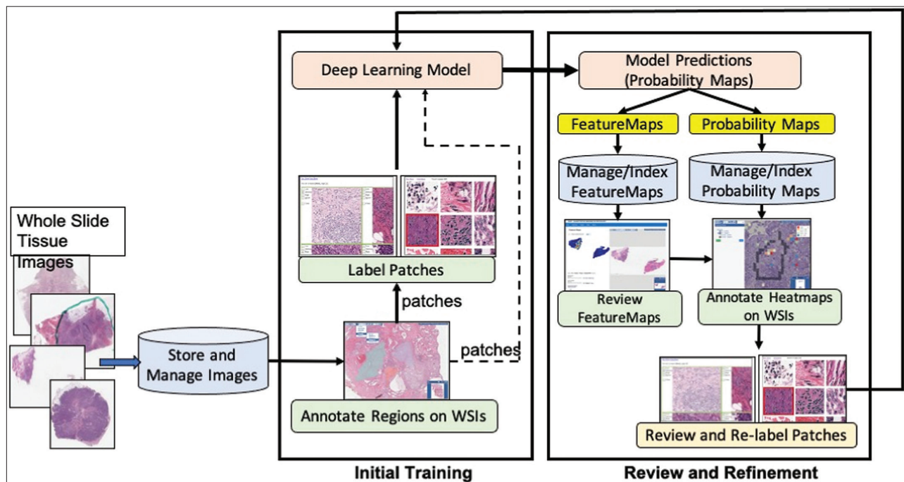
Figure 5: The iterative workflow starts with a set of patches which are extracted from whole slide tissue images and labeled for initial model training. Predictions from the trained model are reviewed as feature maps and heatmaps. The heatmaps are annotated to generate additional labeled patches which are added to the training dataset. The deep learning network is retrained with the updated training dataset to refine the model
