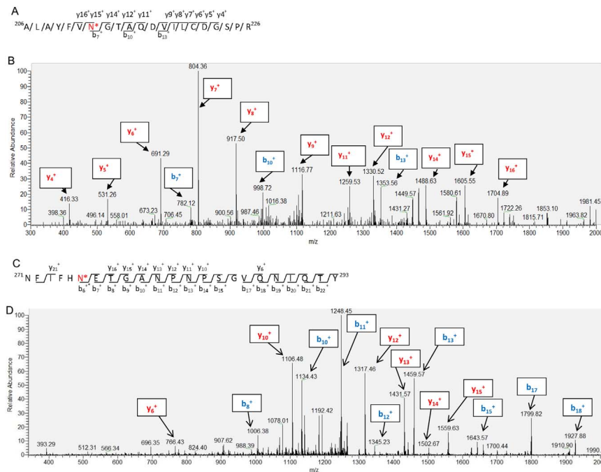
Fig. 3. a Glycosylation peptide (ALAYFVN*GTAQDVILCDGSPR) of IBV S protein following PNGase F treatment of purified IBV. N* represents N-glycosylation site. Identities of the b-ions and y-ions in the spectrum shown in (b). b LC-MS/MS spectrum of the glycosylation peptide in (a) with a [M + 2 H] 2+ precursor ion at 1136.08 m/z. c Another glycosylation peptide (NFIFHN*ETGANPNPSGVQNIQTY) of IBV S protein following PNGase F treatment of purified IBV. N* represents N-glycosylation site. Identities of the b-ions and y-ions in the spectrum shown in (d). d LC-MS/MS spectrum of the glycosylation peptide in (c) with a [M + 2 H] 2+ precursor ion at 1283.61 m/z.
