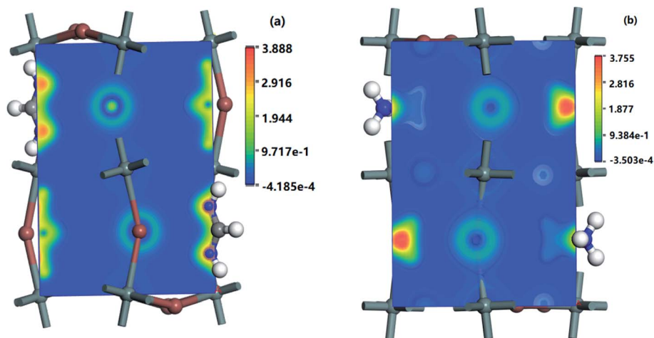
Fig. 7 Charge difference densities of some CBM and VBM bands of (a) \text{MASnI}_3 (110) surface and (b) \text{FASnI}_3 (110) surface.
