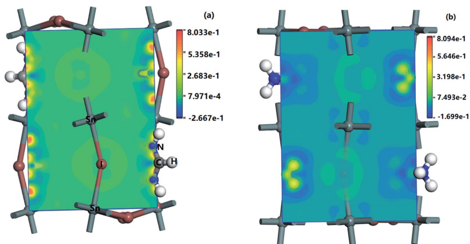
Fig. 6 Charge density of \text{MASnI}_3 and \text{FASnI}_3 , (a) the left panel is \text{MASnI}_3 (110) surface's charge density, (b) the right panel is \text{FASnI}_3 (110) surface's charge density.
