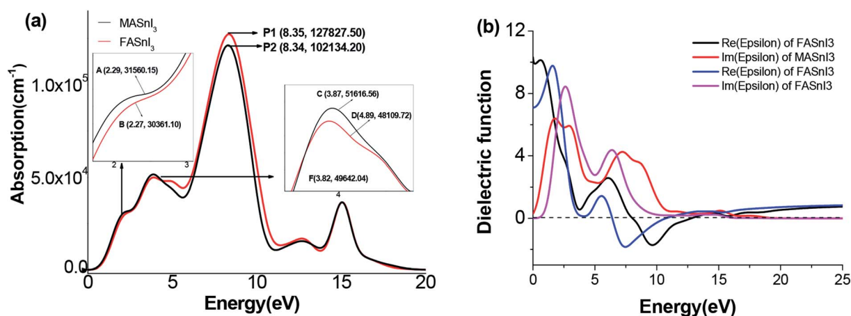
Fig. 8 Calculated (a) absorption spectra and (b) dielectric spectra of the \text{MASnI}_3 and \text{FASnI}_3 systems. In the dielectric spectra, the imaginary parts are shown in red lines, and the real parts are shown in black and bulk lines.
