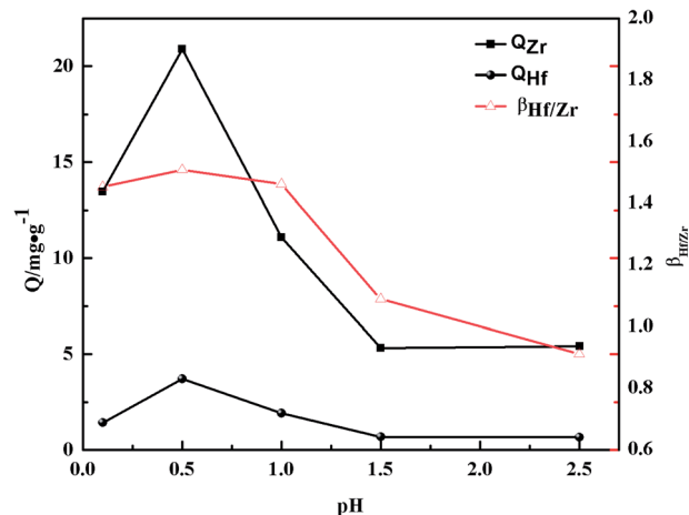
Fig. 6 The effects of acidity on the adsorption capacity Q and separation factors \beta_{Hf/Zr} of Zr(IV) and Hf(IV) on the PS-G1.0-MSNs sorbent.
