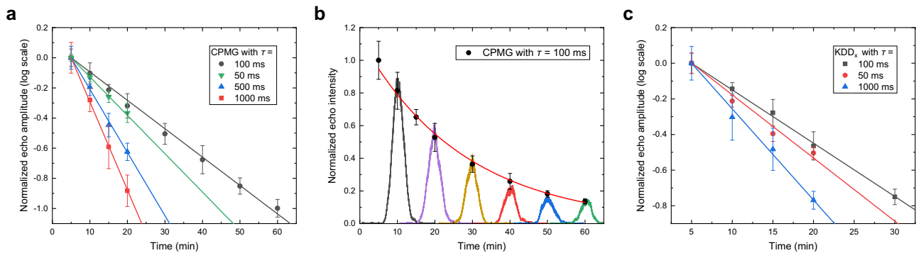
Fig. 3 Measurements of the memory lifetime. a , c Decay of the spin-wave AFC echo with the CPMG and \text{KDD}_x sequences, respectively. The two DD sequences reach their longest storage lifetime of 52.9 \pm 1.2 and 33.3 \pm 1.1 min with a period \tau = 100 ms. b The decay of the echo intensity using CPMG with \tau = 100 ms versus the storage time. Some of the single-shot oscilloscope traces of the read out signals are included. Each data point is averaged four times. The error bars indicate one standard deviation of the echo area.
