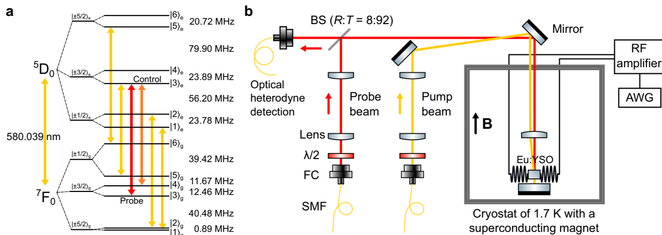
Fig. 1 Energy level diagram and experimental setup. a The laser at 580.039 nm is resonant with electronic state ^5D_0 and ^7F_0 of ^{151}\text{Eu}^{3+}:\text{Y}_2\text{SiO}_5 , which split into six hyperfine levels respectively in the ZFZO magnetic field. |3\rangle_g , |4\rangle_g , and |3\rangle_e form the \Lambda system for the long-lived spin-wave AFC storage. Details about the hyperfine structure and the pumping scheme can be found in the Supplementary Note 2. The AFC is prepared in the |3\rangle_g level. The control pulse resonant with the |4\rangle_g and |3\rangle_e transfers the optical coherence into a spin wave and drives the spin wave back to the optical regime. b Schematic of the experimental setup. The probe and pump beam are emitted with single-mode fibers (SMF) and fiber collimators (FC) before entering the cryostat. The two beams are arranged in a non-collinear configuration. Half-wave plates ( \lambda/2 ) control the polarization of the beams, and two pairs of lenses are used to obtain proper beam widths at the position of the crystal. A BS (beam splitter) with a reflection-to-transmission ratio of 8:92 is employed to efficiently collect the transmitted signal. The probe beam is reflected by the mirror at the bottom of the cryostat and coupled to a SMF for optical heterodyne detection after passing through the BS. A pair of coils placed at the two sides of the sample is driven by an arbitrary waveform generator (AWG) with the output amplified with a 300-W RF amplifier.
