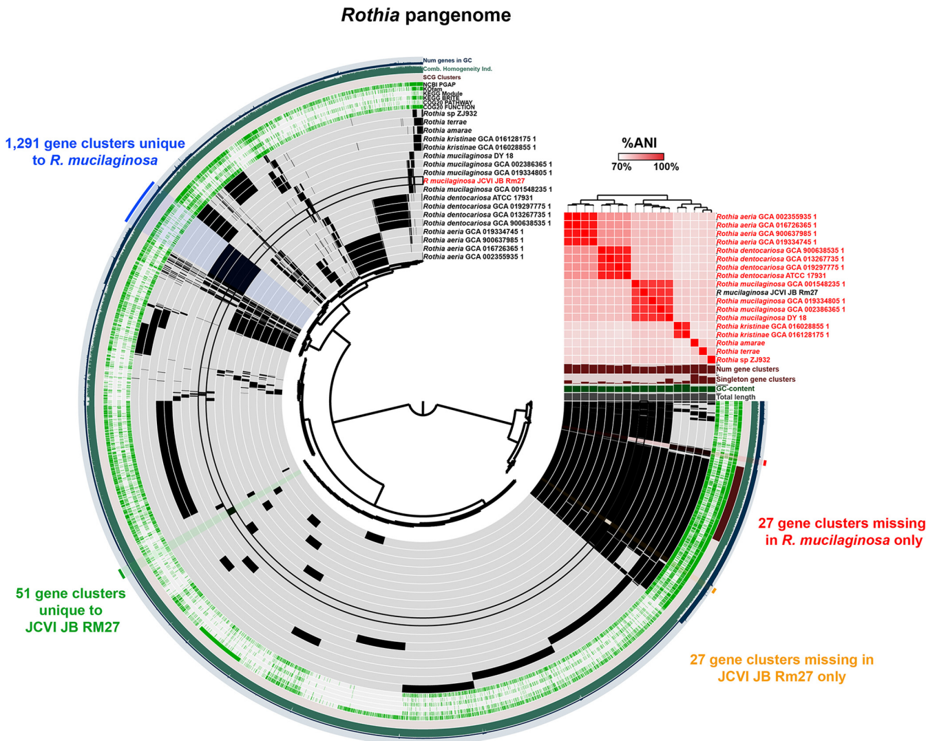
FIG 5 The Rothia pangenome. The dendrogram in the center organizes the 8,118 gene clusters identified across the indicated genomes represented by the innermost 18 layers. The data points within these 18 layers indicate the presence of a gene cluster in a given genome. From inside to outside, the next 6 layers indicate known versus unknown COG function, COG pathway, KEGG Brite, KEGG module, KOfam, and NCBI PGAP annotation. The next 4 layers indicate single copy core gene (SCG) clusters, the combined homogeneity index, the number of genes in the gene cluster, and the number of contributing genomes. The outermost layer indicates the gene clusters present in the following groups: gene clusters missing in only R. mucilaginosa , gene clusters unique to R. mucilaginosa , gene clusters unique to JCVI-JB-Rm27, and gene clusters missing in only JCVI-JB-Rm27. The 18 genome layers are ordered based on the tree of the %ANI comparison, which is displayed with the red and white heat map. The layers underneath the %ANI heat map, from top to bottom, indicate number of gene clusters, number of singleton gene clusters, GC content, and total length of each genome.
