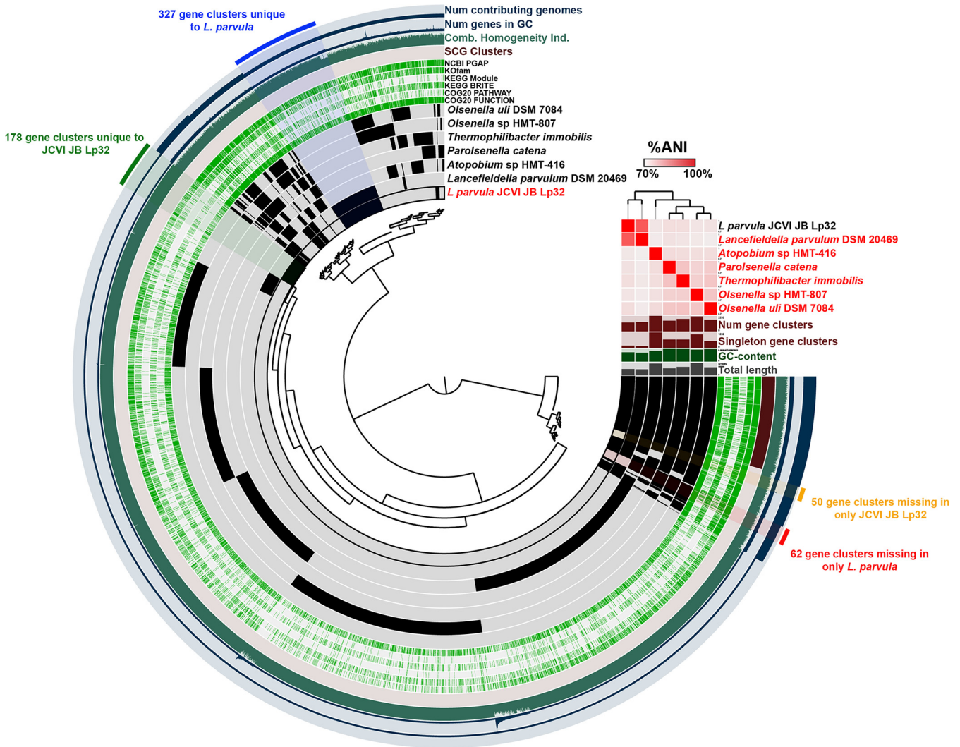
FIG 7 The Atopobiaceae pangenome. The dendrogram in the center organizes the 6,488 gene clusters identified across the indicated genomes represented by the innermost 7 layers. The data points within these 7 layers indicate the presence of a gene cluster in a given genome. From inside to outside, the next 6 layers indicate known versus unknown COG function, COG pathway, KEGG Brite, KEGG module, Kofam, and NCBI PGAP annotation. The next 4 layers indicate single copy core gene (SCG) clusters, the combined homogeneity index, the number of genes in the gene cluster, and the number of contributing genomes. The outermost layer indicates the gene clusters present in the following groups: gene clusters missing in only L. parvula , gene clusters unique to L. parvula , gene clusters unique to JCVI-JB-Lp32, and gene clusters missing in only JCVI-JB-Lp32. The 7 genome layers are ordered based on the tree of the %ANI comparison, which is displayed with the red and white heat map. The layers underneath the %ANI heat map, from top to bottom, indicate: number of gene clusters, number of singleton gene clusters, GC content, and total length of each genome.
