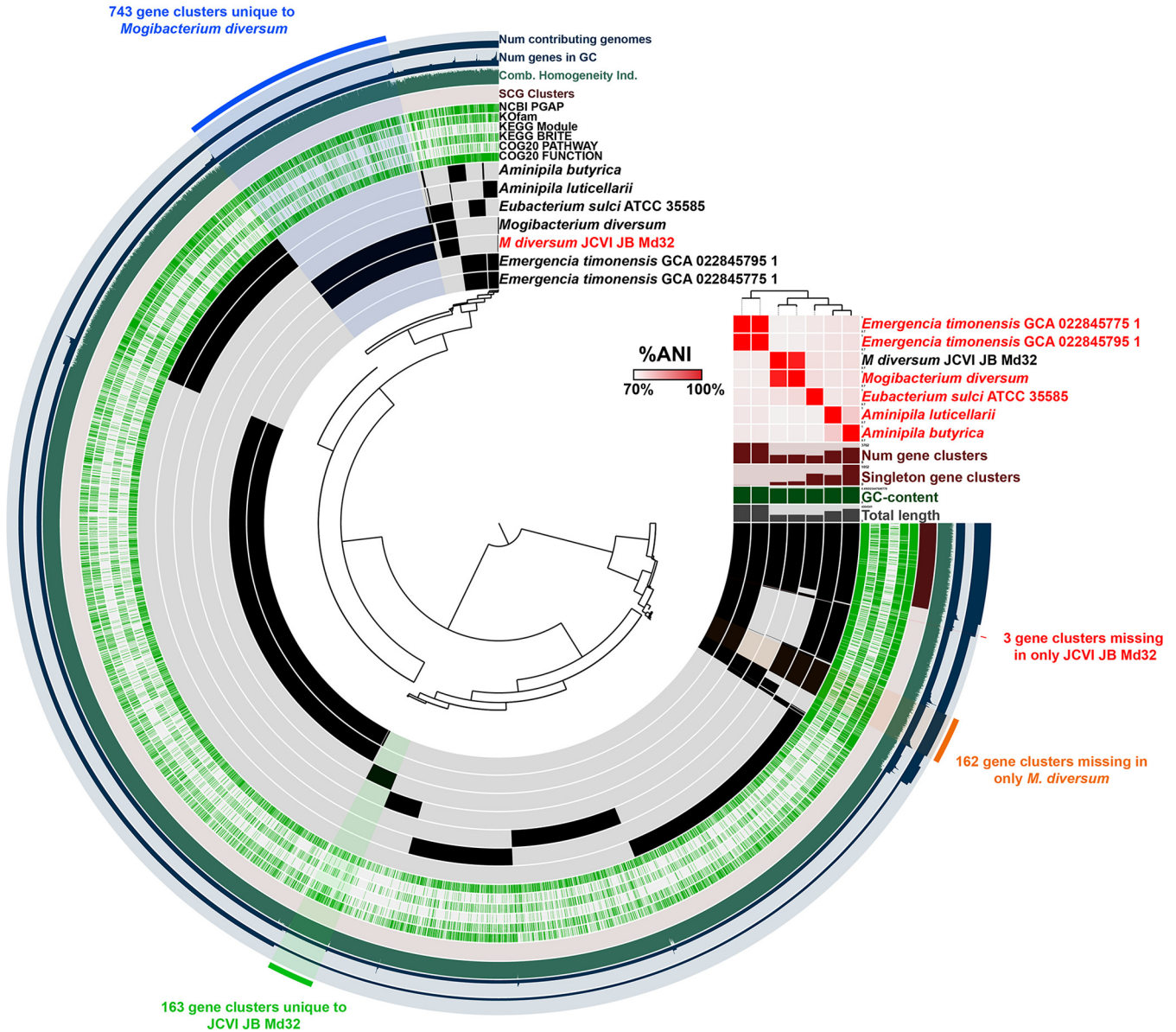
FIG 6 The Eubacteriales Family XIII, insertae sedis pangenome. The dendrogram in the center organizes the 8,084 gene clusters identified across the indicated genomes represented by the innermost 7 layers. The data points within these 7 layers indicate the presence of a gene cluster in a given genome. From inside to outside, the next 6 layers indicate known versus unknown COG function, COG pathway, KEGG Brite, KEGG module, KOfam, and NCBI PGAP annotation. The next 4 layers indicate single copy core gene (SCG) clusters, the combined homogeneity index, the number of genes in the gene cluster, and the number of contributing genomes. The outermost layer indicates the gene clusters present in the following groups: gene clusters missing in only M. diversum , gene clusters unique to M. diversum , gene clusters unique to JCVI-JB-Md32, and gene clusters missing in only JCVI-JB-Md32. The 7 genome layers are ordered based on the tree of the %ANI comparison, which is displayed with the red and white heat map. The layers underneath the %ANI heat map, from top to bottom, indicate number of gene clusters, number of singleton gene clusters, GC content, and total length of each genome.
