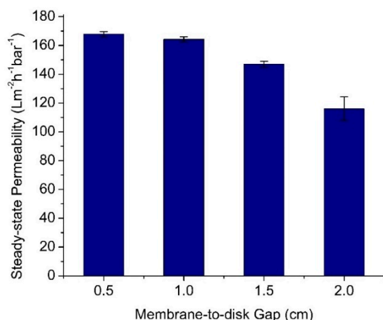
Figure 7. The effect of the membrane-to-disk gap on the permeability. A narrow gap offered a higher hydraulic throughput.
