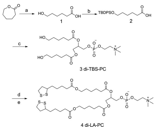
Scheme 2 Synthetic route for di-LA-PC conjugate. Reagents and conditions: (a) NaOH/H 2 O, rt, 12 h, 98%; (b) TBDPSCI, imidazole, DMF, 0 °C to rt, 8 h, 67%; (c) L-α-glycerophosphorylcholine, CDI, DBU, CH 2 Cl 2 , DMSO, rt to 45 °C, 12 h, 71%; (d) TBAF, THF, rt, 4 h, 96%; and (e) lipoic acid, DCC, DMAP, CH 2 Cl 2 , 35 °C, 23%.
