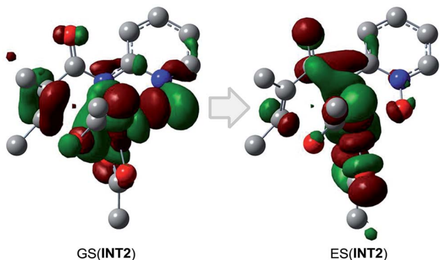
Fig. 1 The lowest excited-state doublet derives from excitation of an \alpha -electron from the singly occupied SOMO (GS(INT2)) into the nominally unoccupied LUMO (ES(INT2), d_{z^2} ). The resulting excited state is 37.2 \text{ kcal mol}^{-1} above the ground state, corresponding to a photon energy of 906.95 \text{ nm} .
