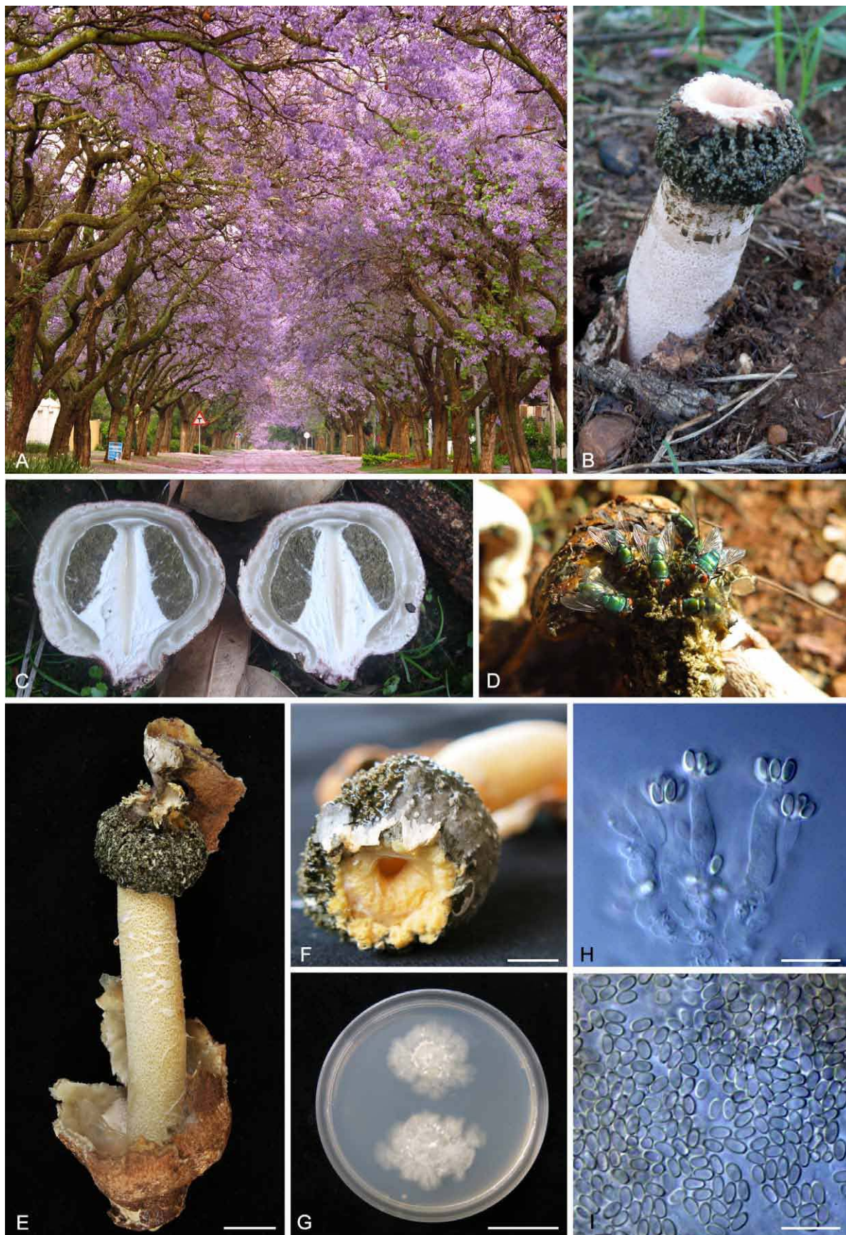
Fig. 1. Habitat and features of Itajahya galepiculata in Pretoria, South Africa. A. Jacaranda mimosifolia trees flowering in Brooklyn, Pretoria. B. Basidiome emerged from the ground (PREM 61269). C. “Egg” dissected to show inner features. D. Flies attracted by putrid odour produced by the fungus. E. Basidiome emerged in a moist chamber in the laboratory (PREM 61268). F. Close-up of the apex of basidiome showing calyptra and gleba (PREM 61270). G. Colonies grown for 3 months on 2 % Yeast-malt extract agar (CMW 44300 = CBS 140331). H. Basidia. I. Basidiospores. Bars: E = 1.5 cm, F = 1 cm, G = 2 cm, H–I = 10 \mu m.
