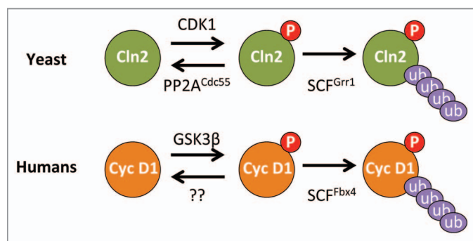
Figure 1. Phosphorylation-dependent degradation of G 1 cyclins in yeast and humans. In yeast, CDK1-dependent phosphorylation of Cln2 leads to Cln2 degradation via SCF Grr1 . This degradation can be inhibited by Cln2 dephosphorylation by the PP2A Cdc55 phosphatase. In humans, GSK3 \beta phosphorylates Cyclin D1, resulting in Cyclin D1 ubiquitination by SCF Fbx4/aB-crystallin .
