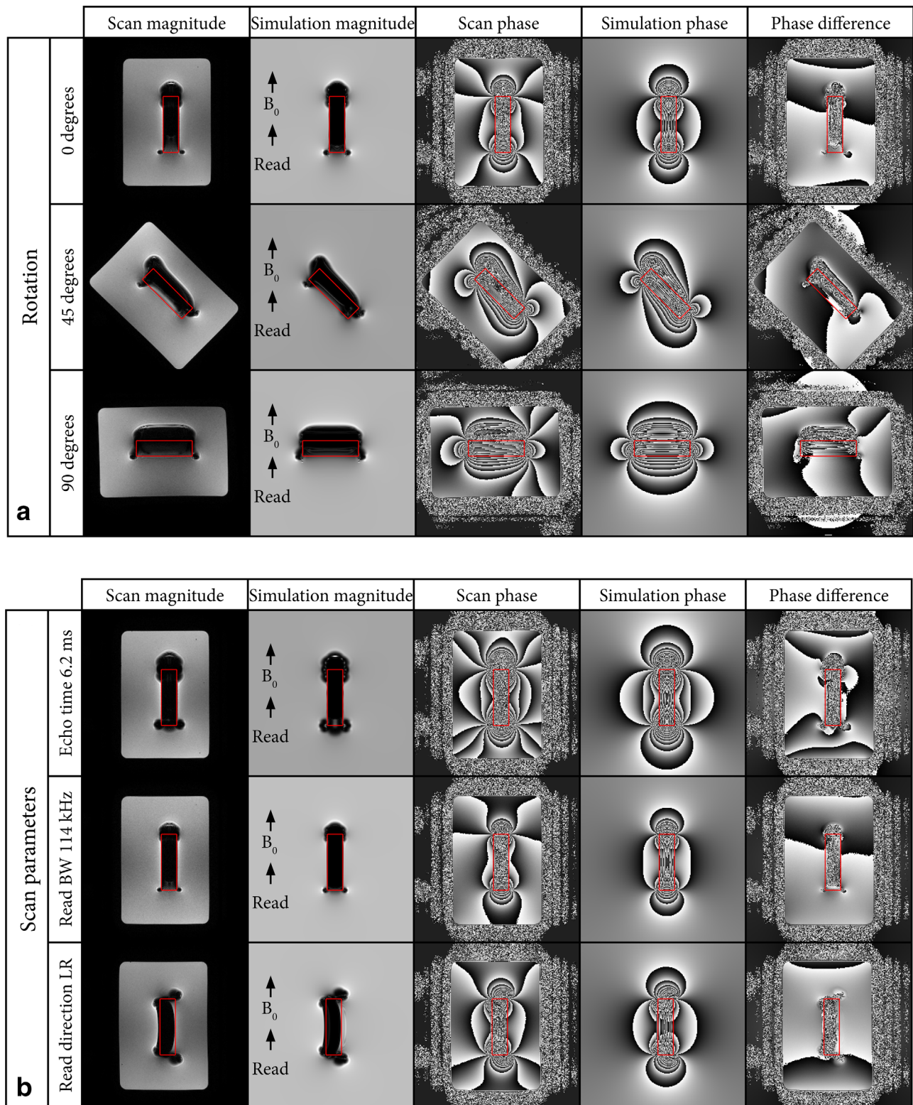
FIG. 1. MRI scans (first and third columns) and FORECAST simulations (second and fourth columns) of a titanium cylinder rotated approximately 0°, 45°, and 90° in the coronal plane (A) and with varying scan parameters (B). Echo time increased to 6.2 ms (fourth row), readout bandwidth increased to ~114 kHz (fifth row), and readout direction changed to left-right (LR) (sixth row). The fifth column shows the difference in phase between the MRI scan and the simulations. The outline of the cylinder is shown in red.
