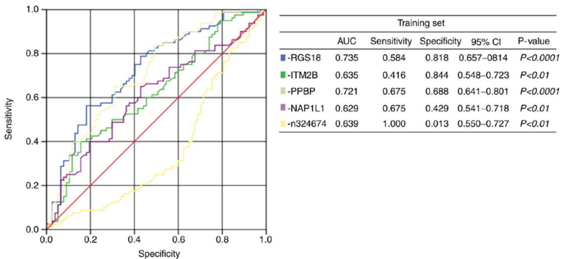
Figure 3. Receiver operating characteristic curve analysis of plasma RNAs: RGS18, ITM2B, PPBP, NAP1L1 and n324674. RGS18, regulator of G-protein signaling 18; ITM2B, integral membrane protein 2B; PPBP, pro-platelet basic protein; NAP1L1, nucleosome assembly protein1-like 1; CI, confidence interval, AUC, area under the curve.
