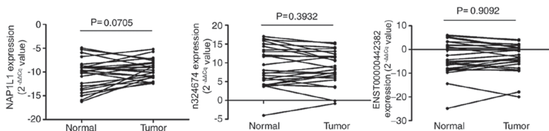
Figure 6. Relative expression levels of NAP1L1, n324674 and ENST00000442382 in 26 gastric cancer and paired normal gastric tissue samples. No significant differences between normal and tumor tissues were observed according to paired t-tests. NAP1L1, nucleosome assembly protein1-like.
