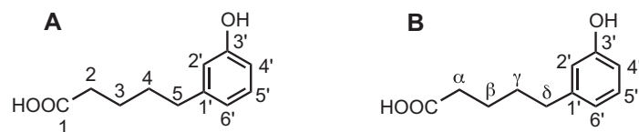
FIGURE 1 Numbering of the phenolic ring and its side chain with the current practice (A) and the older less fashionable use of lowercase Greek letters for the side chain (B).
