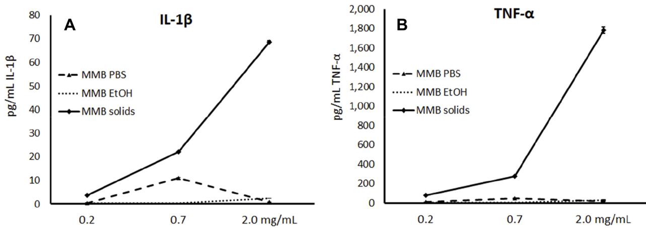
Figure 6 Changes in immune-activating pro-inflammatory cytokine levels in human PBMC cultures. Notes: Changes in Interleukin-1 \beta (IL-1 \beta ), (A) and Tumor Necrosis Factor- \alpha (TNF- \alpha ), (B) cytokine levels in human PBMC cultures treated for 24 hrs with serial dilutions of MMB aqueous extract in PBS (MMB PBS), MMB post-aqueous ethanol extract (MMB EtOH), and the solid fraction (MMB solids). Data are presented as picogram per milliliter (pg/mL) based on the mean \pm standard deviation from triplicate cultures and represents one of three experiments using PBMC from three different healthy human donors. Cytokine levels for LPS-treated control cultures were as follows: IL-1 \beta : 772 \pm 28 pg/mL; TNF- \alpha : 7073 \pm 185 pg/mL.
