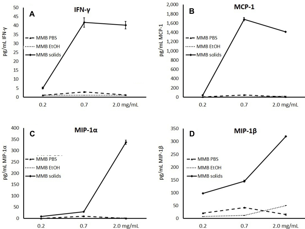
Figure 7 Changes in anti-viral cytokine levels in human PBMC cultures. Notes: Changes in Interferon- \gamma (IFN- \gamma ), (A), Monocyte Chemoattractant Protein-1 (MCP-1), (B), Macrophage Inflammatory Protein- \alpha (MIP-1 \alpha ), (C), and Macrophage Inflammatory Protein- \beta (MIP-1 \beta ), (D) cytokine levels in human PBMC cultures treated for 24 hrs with serial dilutions of MMB aqueous extract in PBS (MMB PBS), MMB post-aqueous ethanol extract (MMB EtOH), and the solid fraction (MMB solids). Data are presented as picogram per milliliter (pg/mL) based on the mean \pm standard deviation from triplicate cultures and represents one of three experiments using PBMC from three different healthy human donors. Cytokine levels for LPS-treated control cultures were as follows: IFN- \gamma : 71 \pm 2 pg/mL; MCP-1: 2052 \pm 35 pg/mL; MIP-1 \alpha : 2116 \pm 0 pg/mL; MIP-1 \beta : 6497 \pm 814 pg/mL.
