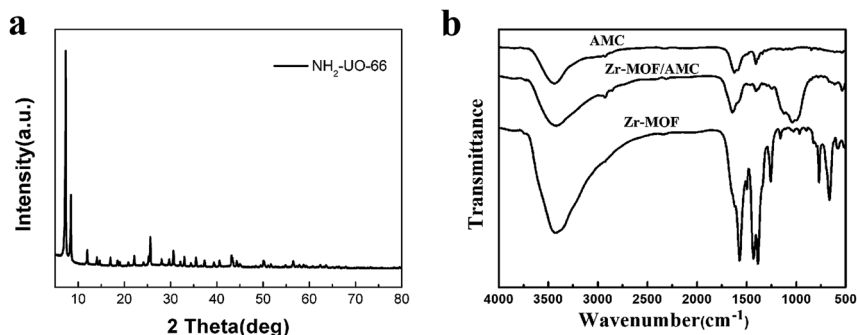
Fig. 1 XRD patterns (a) and FT-IR spectra (b).
