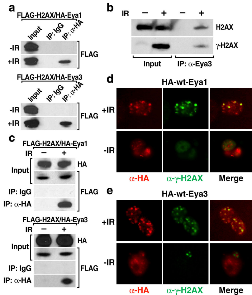
Figure 2. Eya1 and Eya3 interact with H2AX in a DNA-damage dependent manner. (a) HA-tagged Eya1 or Eya3 interacts with FLAG-tagged H2AX in 293T cells in response to IR (5Gy), but not under basal conditions. (b) Co-immunoprecipitation experiments examining endogenous Eya3 protein using a specific Eya3 antibody recapitulated that interaction data for the tagged proteins. (c) Using sonicated chromatin as input, co-immunoprecipitation experiments showed that HA-Eya1/3 interacts with H2AX on chromatin. Immunostaining of 293T cells demonstrates that transfected, HA-tagged Eya1 (d) or Eya3 (e) localizes to DNA-damage induced foci coincident with \gamma H2AX specifically after treatment with IR (5Gy, 1hr). Representative examples of foci formation are shown.
