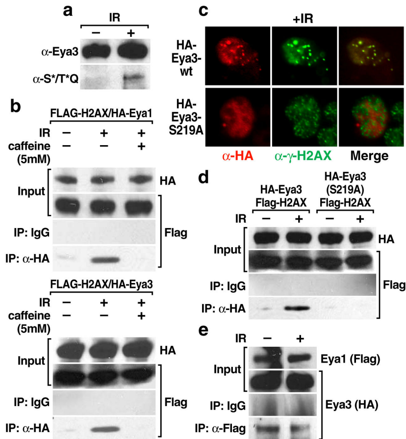
Figure 3. Eya3 phosphorylation by ATM/ATR DNA-damage dependent kinases regulates interaction between Eya and H2AX. (a) Endogenous Eya3 was immunoprecipitated from 293T cells with a specific Eya3 antibody and western blotting was performed with an antibody specific to the phosphorylated target site of ATM/ATR, demonstrating phosphorylation of Eya3 in response to DNA damage (5Gy IR). (b) Eya1/3 interaction with H2AX is lost in the presence of a PI3K inhibitor (5 mM caffeine). (c) Mutation of the ATM/ATR phosphorylation site of Eya3 (S219) prevents formation of damage-induced Eya3 foci. Representative examples of foci formation are shown. (d) HA-Eya3 (S219A) fails to interact with FLAG-H2AX in response to DNA-damage (5Gy IR) by co-immunoprecipitation in 293T cells. (e) DNA damage-independent interaction of Eya3 and Eya1 was assessed by co-immunoprecipitation in 293T cells.
