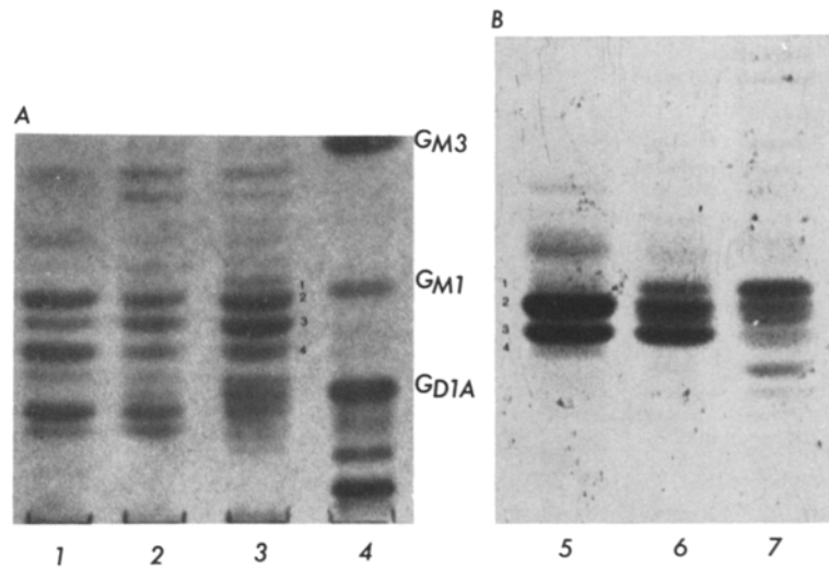
FIGURE 3. High performance, thin layer chromatograms of gangliosides derived from mouse peritoneal macrophages surface labeled by the galactose oxidase/ \text{NaB}^3\text{H}_4 method. Each lane represents the equivalent of 300 \mu\text{g} of cellular protein. (A) Detection of gangliosides by resorcinol-HCl staining. (B) Autoradiogram of the same chromatogram exposed for 7 d. Lanes 1 and 5 are derived from resident macrophages; lanes 2 and 6 are derived from BCG-activated macrophages; lanes 3 and 7 are derived from TG-elicited macrophages; lane 4 contains standard gangliosides derived from bovine brain and these are indicated in the margin. Individual ganglioside species in the \text{GM}_1 region are numbered 1-4.
