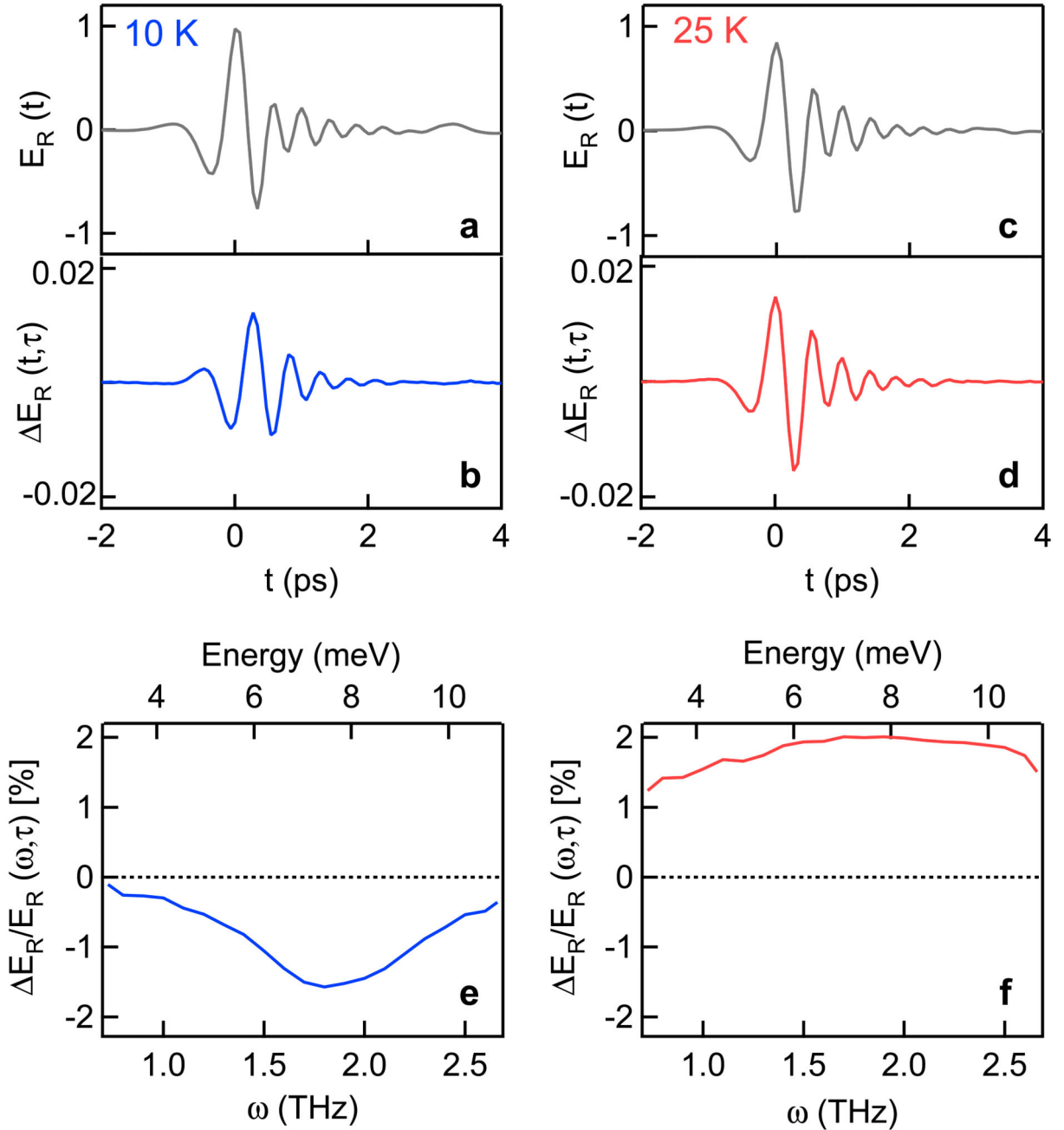
Extended Data Figure 2. “Raw” electric field transients below and above T_c
