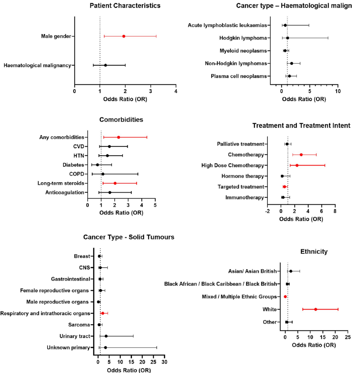
Figure 3. Univariate regression analysis and OR of developing COVID-19, with 95% CIs. Red bars indicate criteria for statistical significance were met ( p < 0.05 ).
