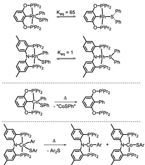
Scheme 1 C–S reductive coupling observed for the (POCOP)Rh(Ph)(SPh) and (PNP)Rh(Ph)(SPh) complexes (ref. 18 and 19, top), C–C coupling with the pincer carbon in (POCOP)Co(Ph)(SPh) (ref. 43, middle), and the subject of this work (bottom).
