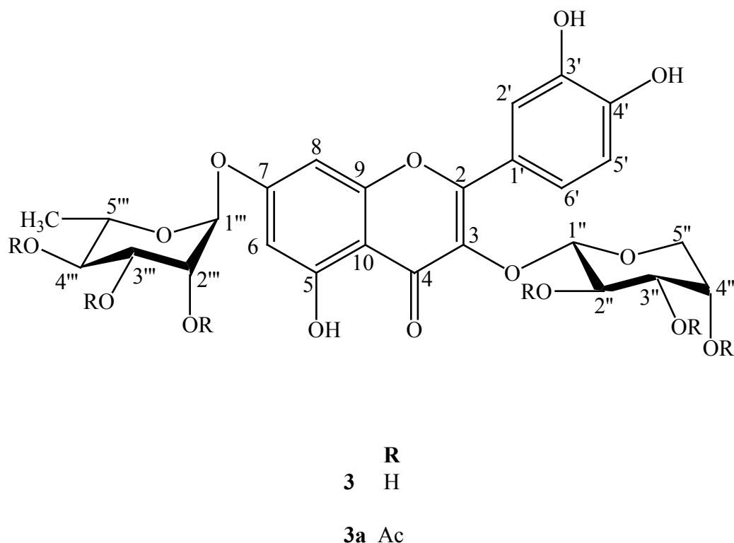
Figure 3. Structure of compounds 3 and 3a.
