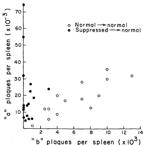
FIG. 2. Development of 7S PFC in irradiated BALB/c recipients of primed cells from (S J L × BALB/c) F 1 (I g a /I g b ) mice. Donor cells were obtained from normal (○) or chronically suppressed (●) heterozygotes immunized 4–105 days previously with 4 \times 10^8 SRBC. A challenge dose of 4 \times 10^8 SRBC was injected together with the primed cells, and the number of antibody-forming cells was determined 7 days later.
