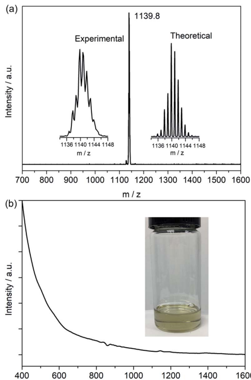
Fig. 1 (a) MALDI-TOF mass spectrum of purified Ti 3 C 3 @I h -C 80 . The insets show the experimental and theoretical isotopic distributions of Ti 3 C 83 . (b) Vis-NIR absorption spectrum of Ti 3 C 3 @I h -C 80 recorded in CS 2 . A photograph of the corresponding solution is shown in the inset.
