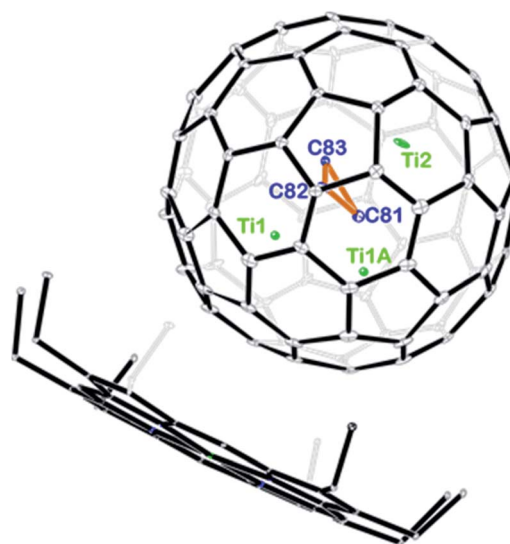
Fig. 2 ORTEP drawing of Ti 3 C 3 @I h -C 80 ·[Ni II (OEP)] with 15% thermal ellipsoids. Only the major Ti 3 C 3 site is shown. Solvent molecules and H atoms are omitted for clarity.
