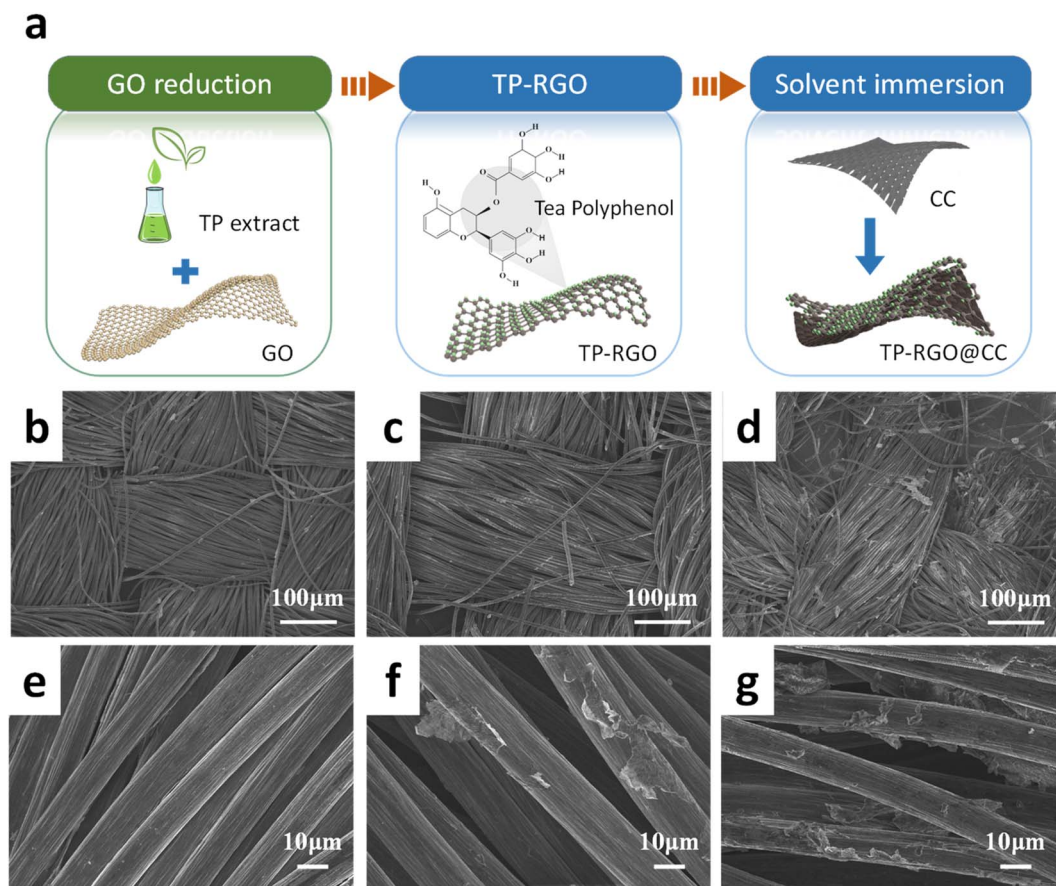
Fig. 1 (a) Schematic illustration for preparation of the TP-RGO@CC anode; SEM images of anodes (b) and (e) CC; (c) and (f) RGO@CC; (d) and (g) TP-RGO@CC.
