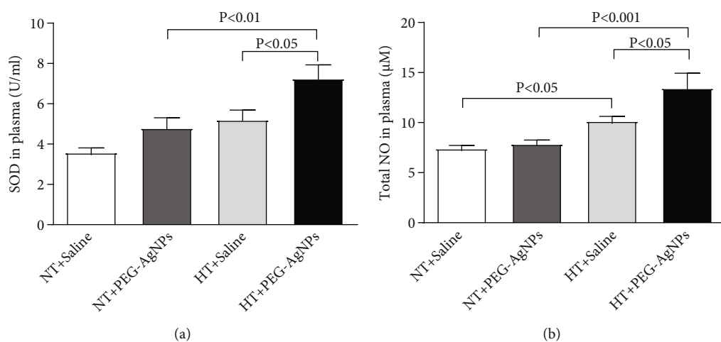
FIGURE 6: Superoxide dismutase (SOD (a)), total nitric oxide (NO (b)) levels in plasma, following intratracheal instillation of saline or polyethylene glycol silver nanoparticles (PEG-AgNPs) in normotensive (NT) or hypertensive (HT) mice. Data are the mean \pm SEM ( n = 6-8 in each group). Statistical analysis by one-way ANOVA followed by Holm-Sidak's multiple comparison test.
