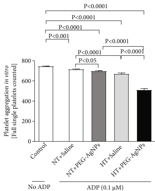
FIGURE 4: In vitro platelet aggregation in whole blood collected from normotensive (NT) or hypertensive (HT) mice after intratracheal (i.t.) instillation of saline or polyethylene glycol silver nanoparticles (PEG-AgNPs). Blood samples obtained from the aforementioned groups were incubated at 37°C with ADP (0.1 μM) for 3 min and stirred for another 3 min, and single platelets were then counted. The degree of platelet aggregation in HT or NT mice exposed to PEG-AgNPs or saline was compared with each other and with that obtained in untreated (without ADP) whole blood obtained from control (unexposed) mice. Data are the mean ± SEM ( n=4 ). Statistical analysis by one-way ANOVA followed by Holm-Sidak's multiple comparison test.
