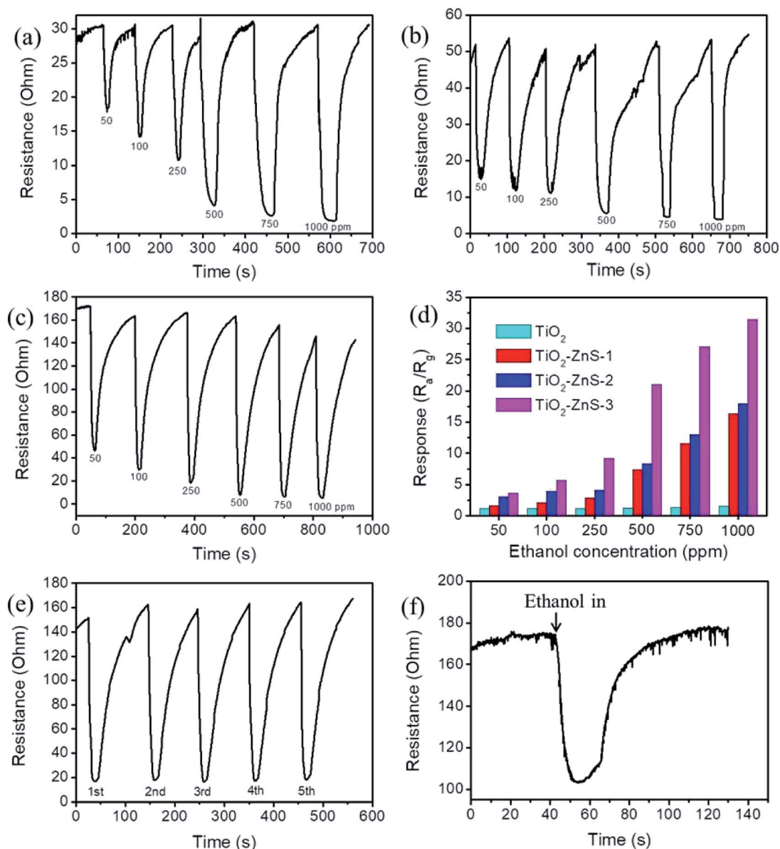
Fig. 8 Dynamic gas-sensing response–recovery curves of the various sensors exposed to different concentrations of ethanol vapor (50–1000 ppm): (a) \text{TiO}_2 -ZnS-1, (b) \text{TiO}_2 -ZnS-2, and (c) \text{TiO}_2 -ZnS-3. (d) Gas-sensing response values comparison of the sensors based on the \text{TiO}_2 , \text{TiO}_2 -ZnS-1, \text{TiO}_2 -ZnS-2, and \text{TiO}_2 -ZnS-3 toward to 50–1000 ppm ethanol vapor. (e) Cycling tests of the \text{TiO}_2 -ZnS-3 sensor on exposure to 250 ppm ethanol vapor. (f) Dynamic gas-sensing response–recovery curve of the \text{TiO}_2 -ZnS-3 sensor exposed to 5 ppm ethanol vapor.
