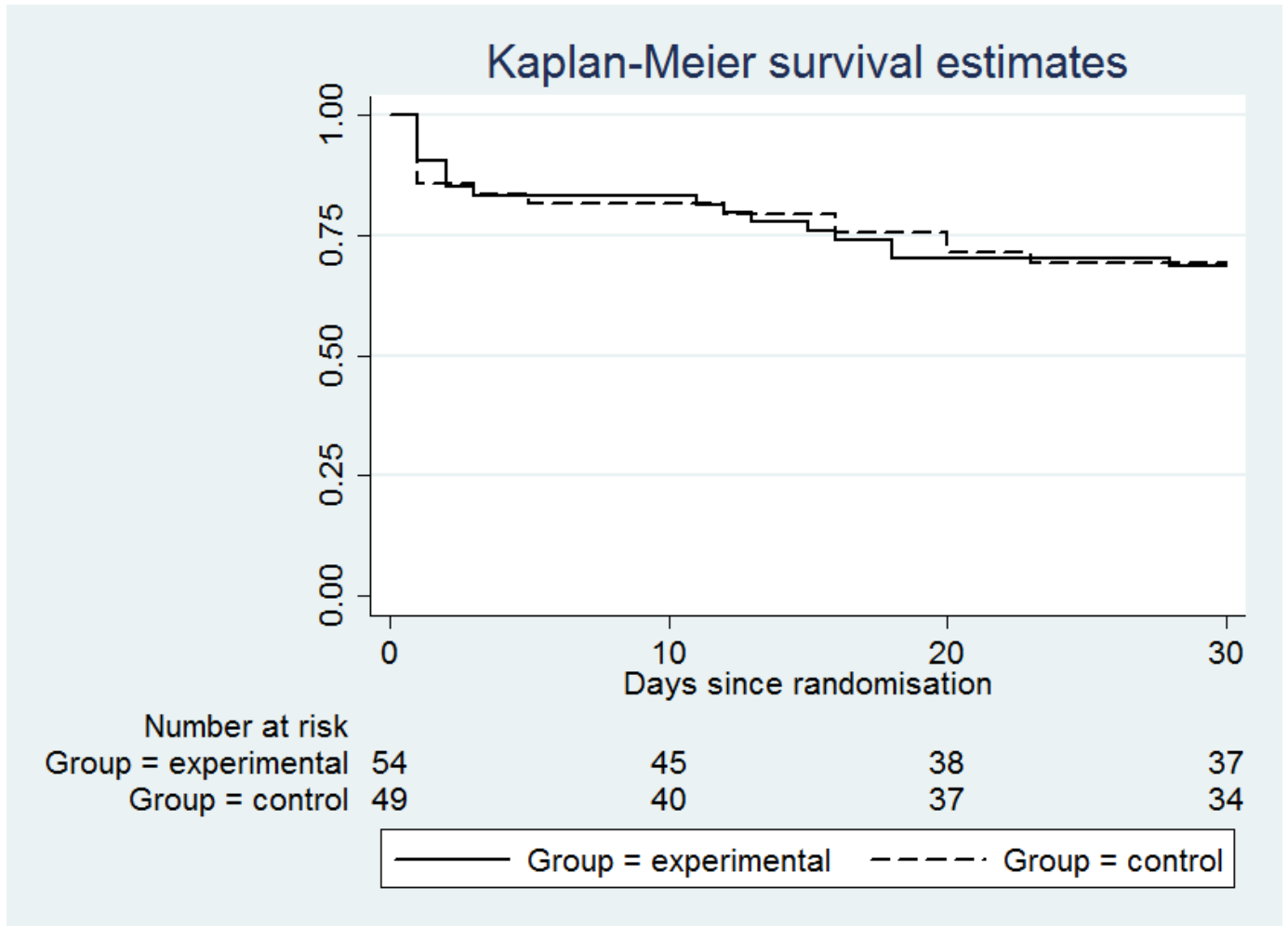
Figure 3 Kaplan-Meier survival estimates. Shown is the probability of survival for participants according to randomisation arm at 30 days.
