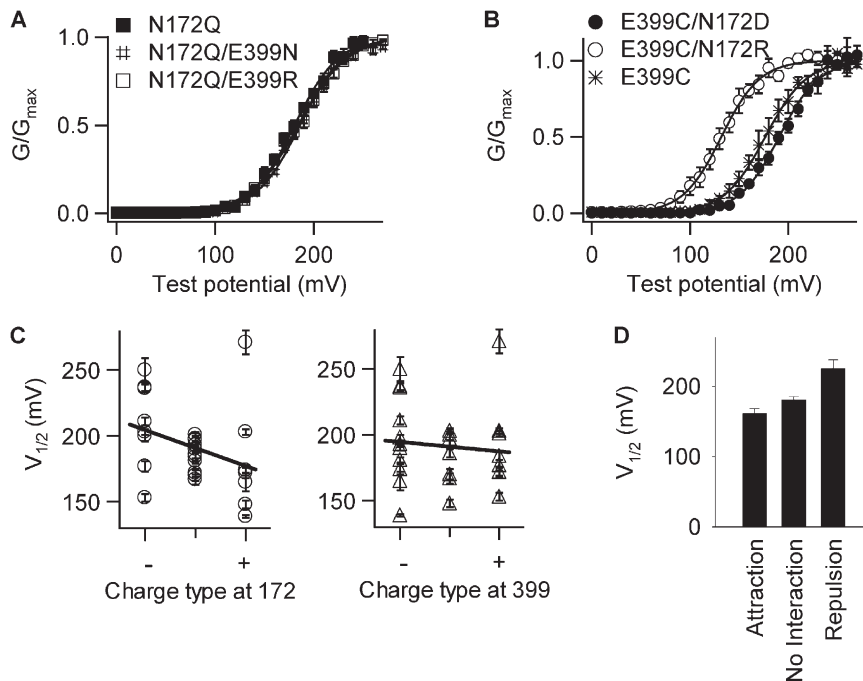
Figure 4. Effects of charge type at residues 172 and 399 on channel activation. G-V relation is shifted by charge type at residue 172 (B) but not by residue 399 (A). [\text{Ca}^{2+}]_i : 0. Solid lines are fittings to the Boltzmann equation. The fitting parameters are: N172Q ( n = 4 ): V_{1/2} = 181 \pm 5 and z = 1.11 \pm 0.20 ; N172Q/E399N ( n = 5 ): V_{1/2} = 186 \pm 4 and z = 1.15 \pm 0.18 ; N172Q/E399R ( n = 5 ): V_{1/2} = 184 \pm 4 and z = 1.04 \pm 0.17 ; E399C/N172D ( n = 8 ): V_{1/2} = 188 \pm 4 and z = 1.23 \pm 0.23 ; E399C/N172R ( n = 5 ): V_{1/2} = 132 \pm 5 and z = 1.30 \pm 0.29 ; E399C ( n = 6 ): V_{1/2} = 201 \pm 4 and z = 1.23 \pm 0.22 . (C) V_{1/2} of a variety of N172 and E399 mutations with or without chemical modifications listed in Table 1 versus charge type at 172 (left) or 399 (right). Solid lines are fittings to linear regression. The slope \pm fitting SD of linear regression is -16.1 \pm 7.5 for the charge type at 172 and -2.6 \pm 7.4 for the charge type at 399. (D) V_{1/2} 's of mutations in Table 1 are averaged based on the interaction type between 172 and 399.
