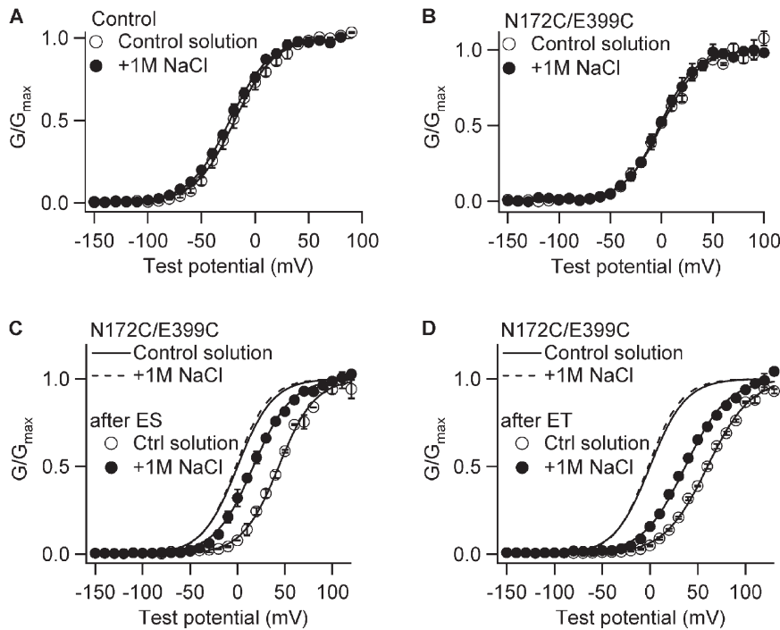
Figure 3. Electrostatic interactions between residues 172 and 399 depend on ionic strength. (A–D) G-V relations in control solution (200 \mu M [\text{Ca}^{2+}] , solution) or in control solution with an additional 1 M NaCl for the control (A), N172C/E399C (B), N172C/E399C after MTSES (C), or N172C/E399C after MTSET (D). All G-V curves are fitted to the Boltzmann equation (lines). The fitting parameters are: the control channel under control solution ( n = 6 ): V_{1/2} = -19 \pm 4 and z = 1.48 \pm 0.08 ; under an additional 1 M NaCl ( n = 3 ): V_{1/2} = -24 \pm 3 and z = 1.36 \pm 0.08 ; N172C/E399C under control solution ( n = 7 ): V_{1/2} = 2 \pm 7 and z = 1.20 \pm 0.09 ; under an additional 1 M NaCl ( n = 8 ): V_{1/2} = 3 \pm 7 and z = 1.32 \pm 0.07 ; N172C/E399C after MTSES under control solution ( n = 2 ): V_{1/2} = 43 \pm 1 and z = 1.32 \pm 0.11 ; under an additional 1 M NaCl ( n = 3 ): V_{1/2} = 17 \pm 2 and z = 1.29 \pm 0.05 ; N172C/E399C after MTSET under control solution ( n = 4 ): V_{1/2} = 60 \pm 1 and z = 1.13 \pm 0.03 ; under an additional 1 M NaCl ( n = 4 ): V_{1/2} = 39 \pm 2 and z = 1.14 \pm 0.03 . The control and N172C/E399C mutation are on the background of C430A.
