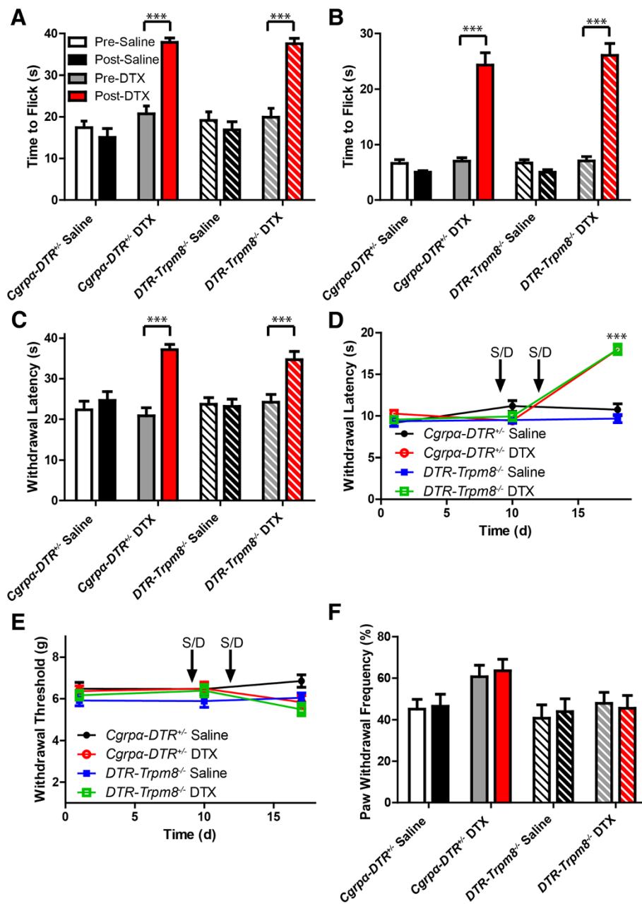
Figure 4 Ablation of CGRP \alpha sensory neurons in DTR-Trpm8 -/- mice reduces heat sensitivity without affecting mechanical sensitivity.
