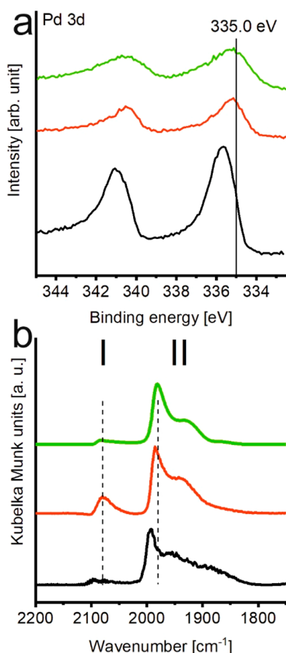
Figure 2. Evaluation of the surface oxidation state of Pd nanoparticles of L-titanate@Pd@L-titanate (black), Pd ext @P25 (red), and Pd ext @Al 2 O 3 (green): (a) XPS spectra of the Pd 3d region; (b) CO DRIFT spectra recorded at room temperature after saturation of the surface at 60 mbar of CO partial pressure followed by outgassing to 2 mbar.
