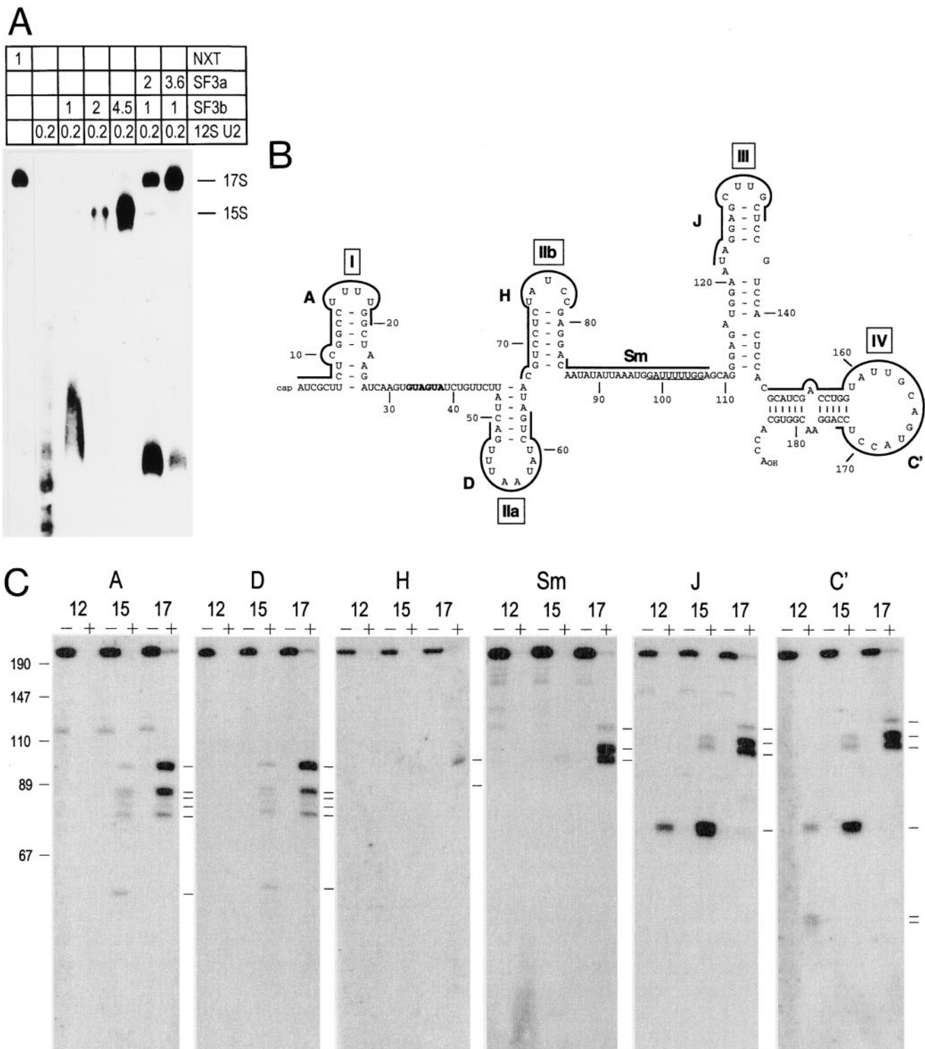
Figure 4. Analysis of micrococcal nuclease-resistant regions in U2 snRNA in the 12S, 15S, and 17S U2 snRNPs. (A) In vitro reconstitution of the 15S and 17S U2 snRNPs. The indicated amounts (in microliters) of nuclear extract (NE), SF3a, SF3b, and the 12S U2 snRNP were incubated with 5' end-labeled oligonucleotide U2A and separated in a 4% polyacrylamide gel. The position of the 15S and 17S U2 snRNPs is indicated on the right. (B) Secondary structure of mammalian U2 snRNA (according to Ares and Igel, 1990; Hartshorne and Agabian, 1990). The Sm-binding site is underlined, the branch site interaction sequence is shown in bold, and the stem-loops are indicated by roman numerals. Sequences complementary to oligonucleotides are shown by thick lines. (C) Analysis of protected fragments of U2 snRNA in the 12S, 15S, and 17S particles by Northern blotting. The 12S U2 snRNP (Mono Q) and reconstituted 15S and 17S U2 snRNPs were incubated in the absence (-) or presence (+) of micrococcal nuclease for 10 min at 30°C. RNA was isolated, separated in a 14% polyacrylamide/8.3 M urea gel, and blotted onto a nylon membrane, followed by detection with oligonucleotides complementary to different portions of U2 snRNA as indicated above each panel. The migration of DNA length markers is indicated on the left of the figure. Please note that the DNA fragments migrate faster than the RNA fragments. Protected U2 snRNA fragments are indicated by lines on the right side of each panel.
