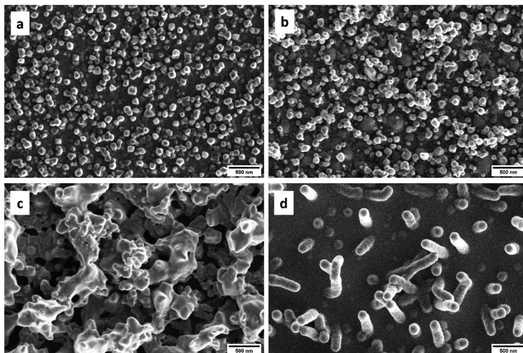
Fig. 5 SEM photographs of thin films grown on Al 2 O 3 (0001) at 500 °C using the different precursors 1–4.
