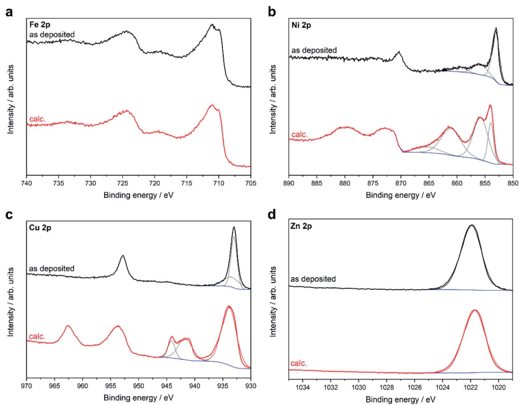
Fig. 6 XPS core level metal 2p spectra of thin films grown on Al 2 O 3 (0001) at 500 °C using the different precursors 1–4 before (as deposited) and after calcination (calc.).
