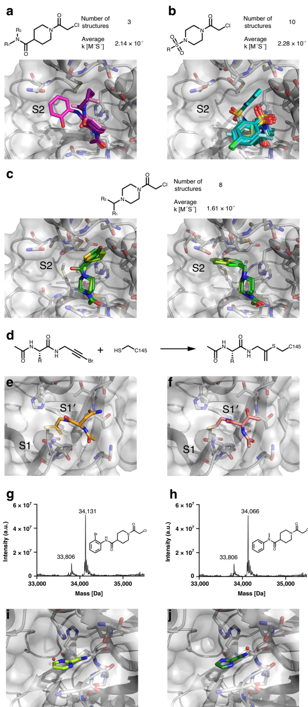
Fig. 6 Covalent fragments are anchored at Cys145 and sample different regions of the orthosteric MPro binding pocket. a Fragments containing N -chloroacetyl piperidiny-4-carboxamide motif. b Fragments containing N -chloroacetyl- N' -sulfonamido-piperazine motif. c Fragments containing N -chloroacetyl- N' -carboxamido- and N -chloroacetyl- N' -heterobenzyl-piperazine in two binding modes. The second order kinetic constants refer to the intrinsic thiol reactivity of these fragment hits as previously measured 29 . d Reaction schema of the unexpected covalent modification to Cys145 by PepLites hits. e Threonine PepLite (NCL-00025058 (x0978)) bound covalently to active site cysteine. f Asparagine PepLite (NCL-00025412 (x0981)) bound to active site cysteine. Labelling of MPro by 2nd generation compounds proven by intact protein LC-MS: g Labelling by PG-COV-35; h Labelling by PG-COV-34. Covalently bound cyclic electrophiles: i Cov_HetLib 030 (x2097) and j Cov_HetLib 053 (x2119).
