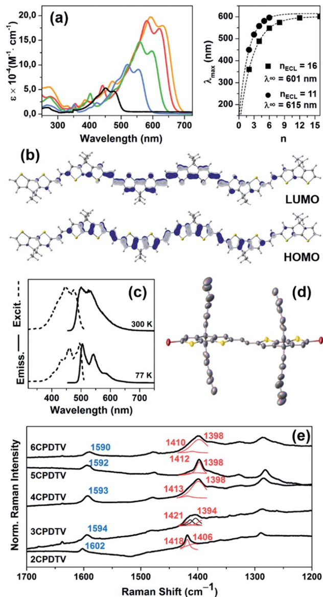
Fig. 1 (a) Left: UV-Vis absorption spectra of n CPDTV in \text{CH}_2\text{Cl}_2 . Right: Meier's plot fitting for n CPDTV (circles) and n TV series (squares) and their effective conjugation length (ECL) and the absorption maximum of the infinite chain, ( \lambda_\infty ). (b) DFT/B3LYP/6-31G** Frontier molecular orbital for 6CPDTV. (c) Excitation (dashed lines) and emission (solid lines) spectra of 2CPDTV at 77 K and room temperature. (d) X-ray structure of 2CPDTV-Br (50% thermal ellipsoids). (e) Solid-state Raman ( \lambda = 785 \text{ nm} ) spectra of n CPDTV recorded at room temperature. \nu(\text{C}=\text{C})_{\text{vinyli}} in blue, \nu(\text{C}=\text{C})_{\text{CPDT}} in red. The frequencies have been assigned by deconvolution.
