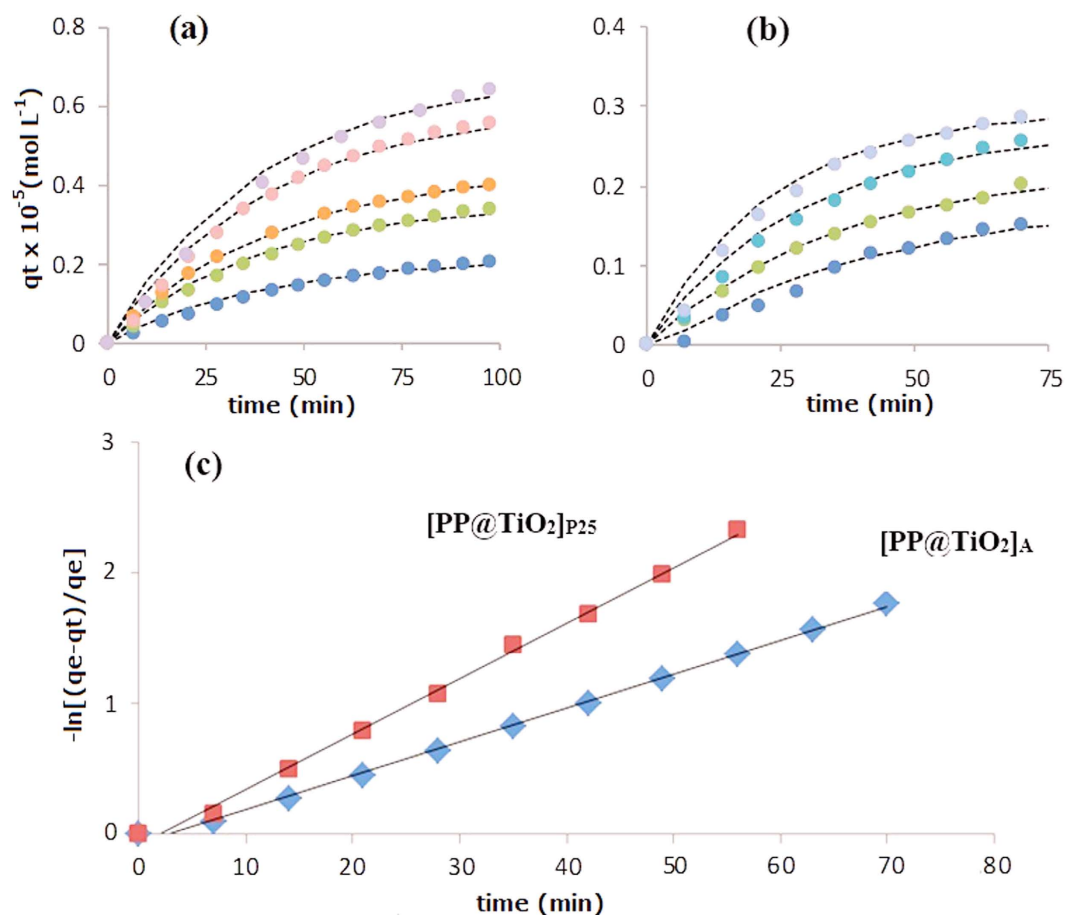
Figure 9. Time evolution of q_t for different initial ARS concentrations for both [\text{PP@TiO}_2]_A (a) and [\text{PP@TiO}_2]_{P25} (b) respectively; pseudo first order adsorption kinetic of ARS ( 7.30 \times 10^{-5} \text{ mol L}^{-1} ) in acidic conditions using [\text{PP@TiO}_2]_A and [\text{PP@TiO}_2]_{P25} respectively (c).
