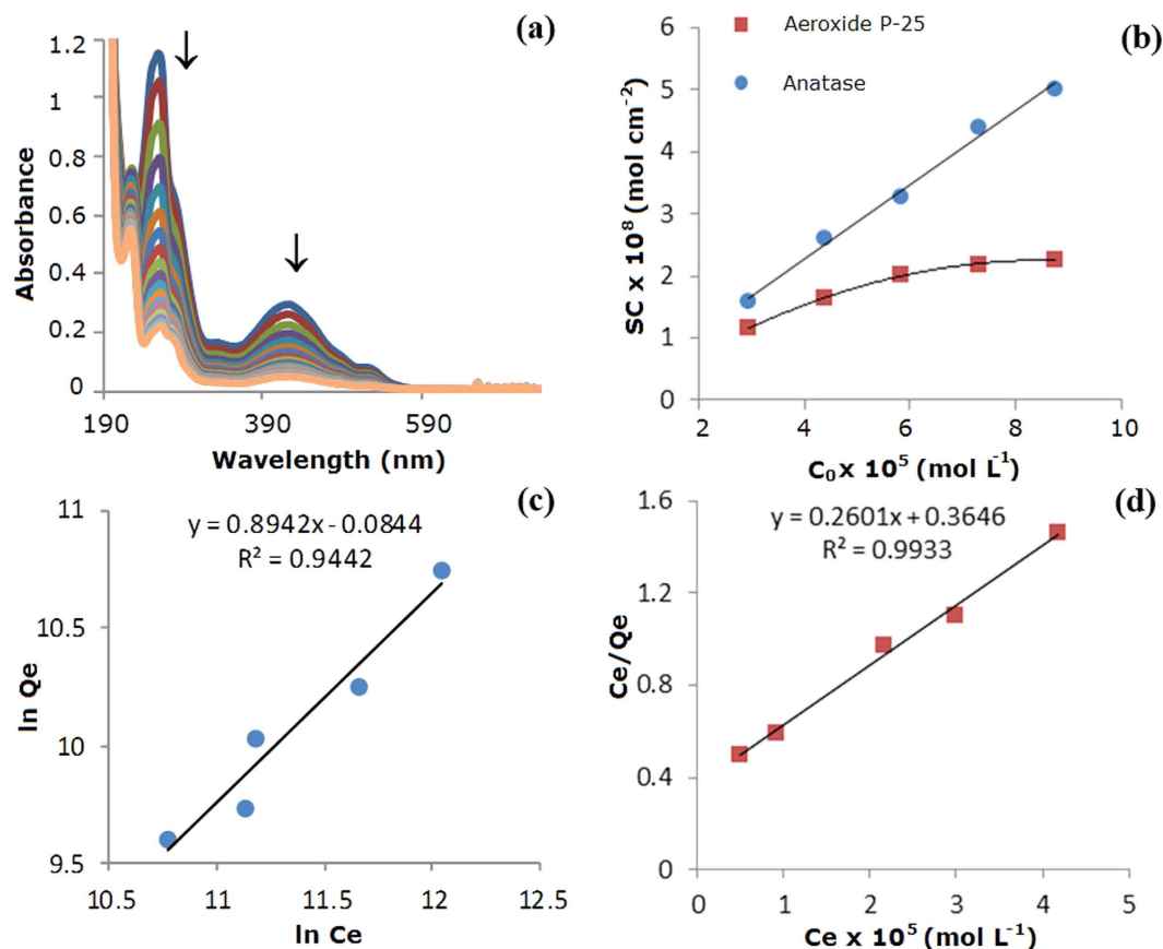
Figure 8. Decrease of UV-Vis spectra in the solution during the adsorption process of 7.30 \times 10^{-5} \text{ mol L}^{-1} of ARS on [PP@TiO 2 ] A (a); surface ARS concentration (SC) increasing ARS solution concentrations from 2.92 \times 10^{-5} to 8.77 \times 10^{-5} \text{ mol L}^{-1} on [PP@TiO 2 ] P25 (red squares) and [PP@TiO 2 ] A (blue dots) (b); isotherm graphs for ARS on [PP@TiO 2 ] A (c) and on [PP@TiO 2 ] P25 (d).
