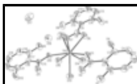
Fig. 1. The molecular structure of the title compound, drawn with 50% probability displacement ellipsoids. H atoms omitted for clarity.
