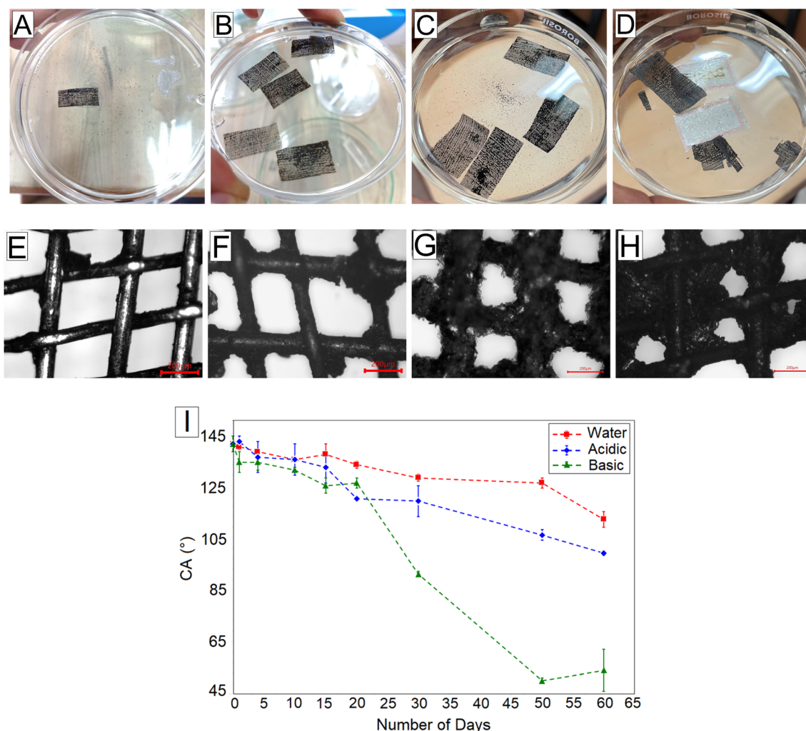
Fig. 5 (A and E) GO-coated mesh immersed in water for 10 days and the corresponding OM image of the mesh after drying. GO*-coated mesh samples immersed continuously for 60 days in (B and F) water, (C and G) acidic medium, and (D and H) basic medium. The scale bar for OM images represents 200 \mu\text{m} . (I) Variation in the underwater edible oil CA when the GO*-coated mesh was immersed in water, acidic medium and basic medium for time durations up to 60 days.
