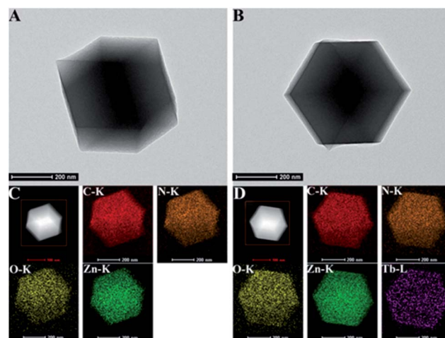
Fig. 2 TEM images of His@ZIF-8 (A) and His@ZIF-8/Tb 3+ (B). Dark field STEM and elemental mapping images of His@ZIF-8 (C) and His@ZIF-8/Tb 3+ (D).
