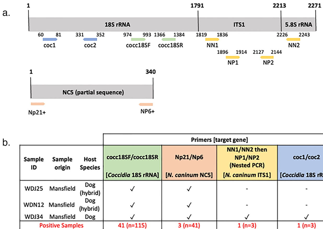
FIGURE 3 PCR amplification of Coccidia and Neospora DNA. (a) Schematic representation of the 18S rRNA, ITS1, 5.8S rRNA and Nc5 locus with relative location of oligonucleotide primers used in this study. Approximate primer position is provided based on Neospora caninum Liverpool strain genome annotation (GenBank accession number U16159) and partial Nc5 (GenBank accession number KP715563). (b) Summary of the PCR screens performed with Coccidian and N. caninum primers
