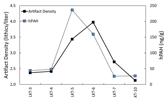
Figure 3. Artifact density of plotted lithic artifacts and hPAH concentrations of each layer at LKT1. Average hPAH concentrations of subunits are nested into their unit designations.
