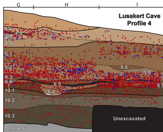
Figure 2. Distribution of measured lithic (red circles) and faunal remains (blue circles) excavated by stratigraphic unit from LKT1 during the 2008–2011 field seasons. 1 meter excavation squares (G, H and I) are labeled. Sedimentary units are labeled in white. Please reference Extended Data Figs 1, 2 for profile location.
