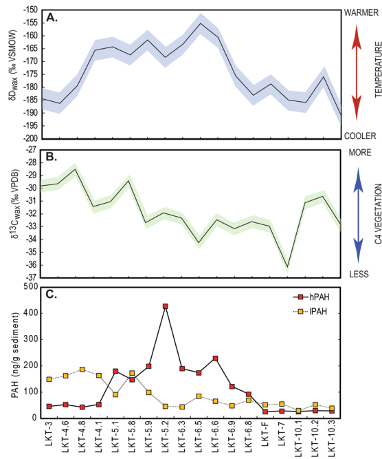
Figure 1. (A) \delta D_{wax} , (B) \delta^{13}C_{wax} , (C) concentrations of hPAHs (red squares), and iPAHs (orange squares) from each sedimentary Unit at LKT1. \delta D_{wax} (4‰) and \delta^{13}C_{wax} (0.5‰) values are plotted with 1\sigma error bars. LKT1 stratigraphic layers are oriented oldest (right) to youngest (left).
