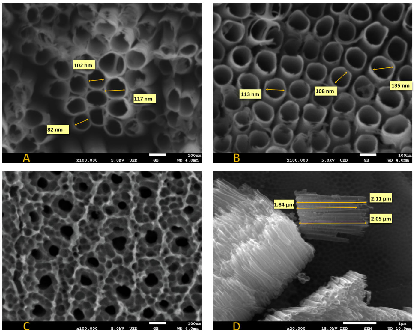
Figure 1. SEM images: (A) pure \text{TiO}_2 nanotubes \text{TiO}_2 -NTs; (B) sample hydrothermally modified \text{Co-TiO}_2 -NTs; (C) sample \text{Co-TiO}_2 after final thermal treatment (450 °C, 2 h); and (D) length of nanotubes for \text{Co-TiO}_2 -NTs.
