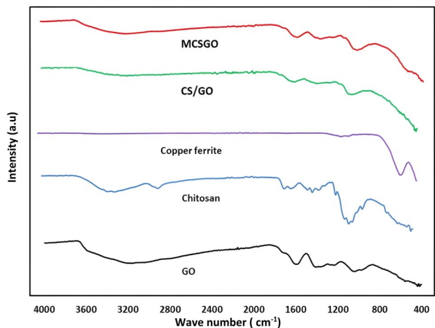
Fig. 2 FTIR spectra of GO, chitosan, CuFe_2O_4 , CS/GO, and MCSGO.
