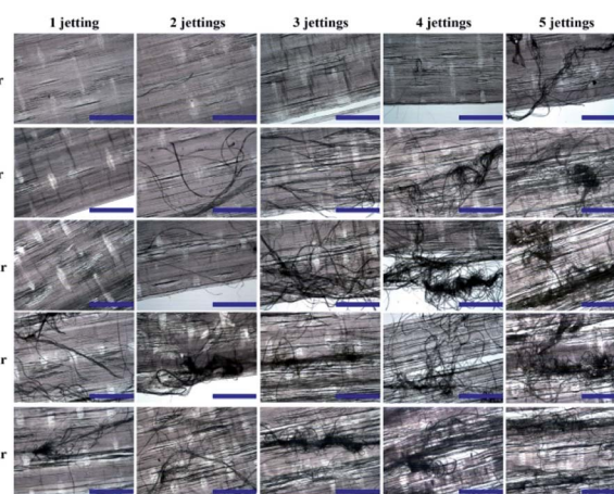
Fig. 5 Light micrographs of MW47 PTFE sintered films split by waterjets with different pressures and manifolds; the blue scale bar is equal to 400 μm.
