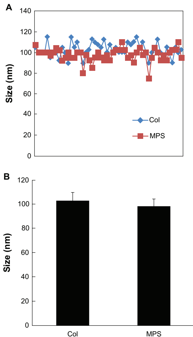
Figure S1 Particle size distribution of MPS and Col NPs. Abbreviations: MPS, mesoporous silica; Col, colloidal silica; NPs, nanoparticles.
