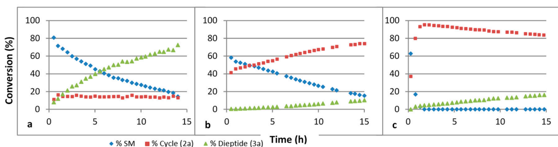
Figure 3. Evolution of a mixture of GlyCN and cysteine in \text{D}_2\text{O} at 45^\circ\text{C} followed by ^1\text{H} NMR, at various pH's. (a) pH 4, (b) pH 6, (c) pH 8. SM: starting materials. Concentration 4 \times 10^{-2} mol/L.
